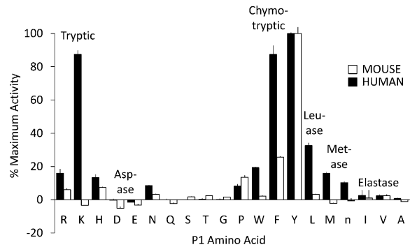
FIGURE 3. Comparison of mouse and human cathepsin G P1 substrate specificity. Purified mouse and human enzymes were profiled using a P1-diverse combinatorial library of fluorogenic tetrapeptide substrates containing all combinations of standard amino acids (except Cys) plus norleucine (n) at positions P2–P4, with each library fixed at P1. Individual assays assess overall ability to hydrolyze tetrapeptides containing a particular P1 amino acid with an equimolar mixture of 8000 peptides varying in 20 residues each in positions P2, P3, and P4 on the N-terminal side of cleavage site P1. To facilitate comparison between human and mouse enzyme, output in fluorescence units is normalized to the percentage of maximum output for each enzyme, which was achieved for both enzymes by the P1 Tyr well. The human enzyme has tryptic, chymotryptic, Leu-ase, and Met-ase activity, without Asp-ase or elastase-like activity, whereas mouse specificity is much narrower and mainly chymotryptic. Error bars show SD ( n = 3 ).
