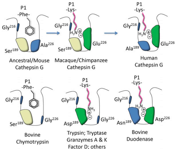
FIGURE 6. Specificity pocket mutations leading to acquisition of tryptic activity. The diagram depicts amino acids of the specificity triad lining the primary specificity pocket of cathepsin G and related serine peptidases, with examples of side chains of substrate P1 residues at the site of hydrolysis. The Ala 226 Glu mutation converted a chymase-like chymotryptic enzyme into a tryptic enzyme capable of hydrolyzing peptides after Lys, as shown, in part due to introduction of the negatively charged Glu side chain, which attracts the positive charge of the P1 Lys \epsilon amino group. Configurations of classic chymotryptic and tryptic peptidases plus bovine duodenase, which uses a different configuration to accommodate tryptic and chymotryptic substrates, are shown for comparison. “Tryptase” refers to mast cell \beta -like tryptases, rather than to human \alpha tryptase, which has an active site blocked by a Gly 216 Asp mutation (60, 61).
