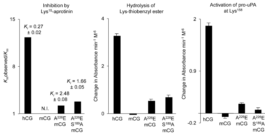
FIGURE 5. Comparison of tryptic (Lys-containing) inhibitor and substrates in wild-type human cathepsin G (hCG), wild-type mouse cathepsin G (mCG), and humanized mutants Ala 226 Glu (A 226 E) and Ala 226 Glu/Ser189Ala (A 226 E/S 189 A) mCG. The left panel compares strength of inhibition, as reflected by the ratio of K_m obtained in the presence ( K_m observed) and absence ( K_m ) of 0.27 \mu M Lys 15 -aprotinin, using the substrate suc-L-Val-Pro-Phe-4NA. K_i units are given in millimolar. The middle panel compares rates of hydrolysis of synthetic tryptic substrate carbobenzyloxy-L-Lys-thiobenzylester (100 \mu M) normalized for peptidase concentration. The right panel compares rates of hydrolysis of human prouPA, which is activated by cleavage at Lys 158 , as assessed by hydrolysis of urokinase plasminogen activator substrate suc-L-Val-Gly-Arg-4NA. N.I., no inhibition.
